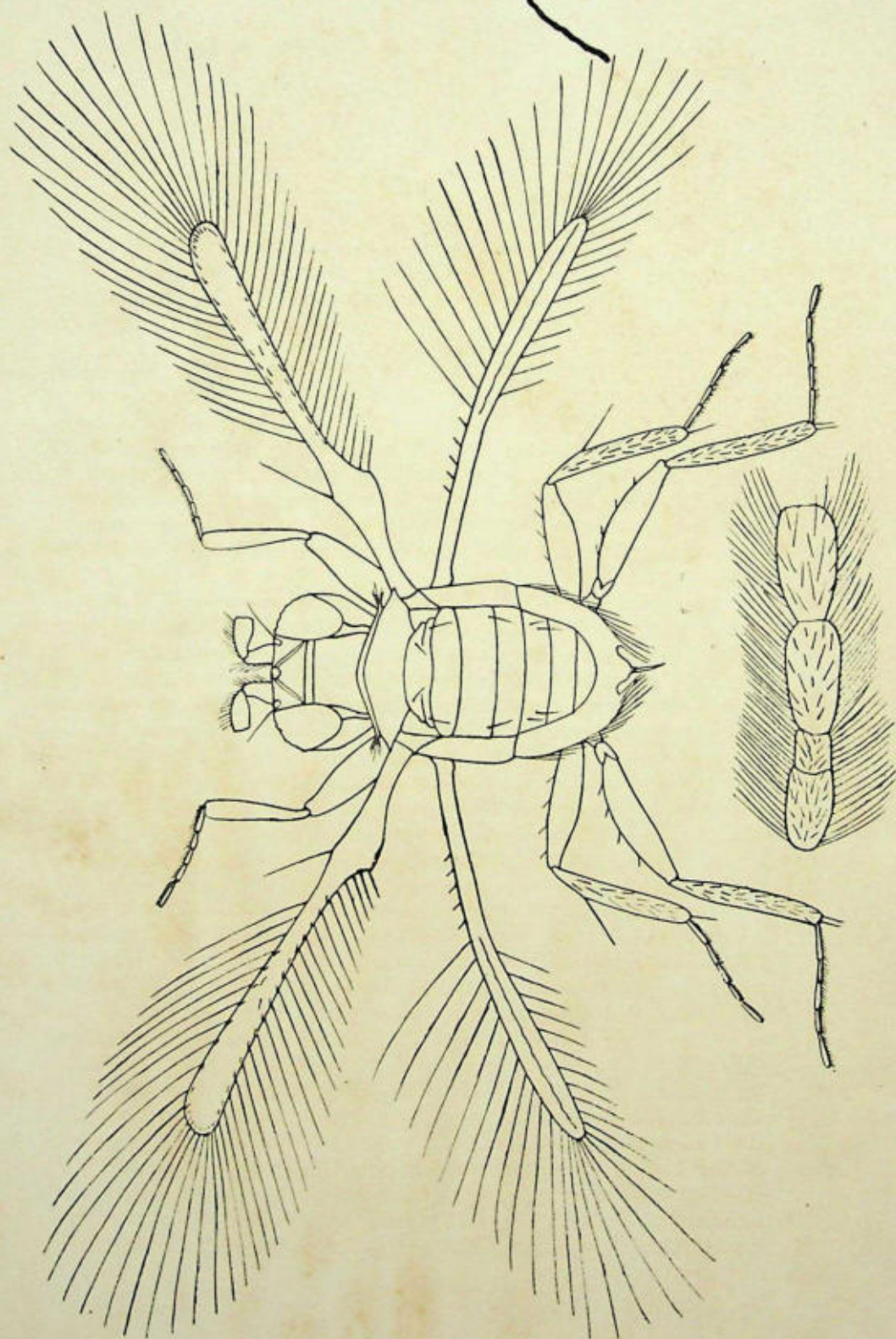
Alaptus magnanimus , ♂, \times 240 , with the third to sixth joints of the antenna more highly magnified.
