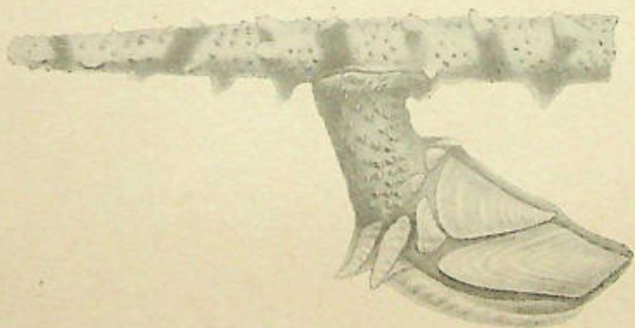
FIG. 1.— Scalpellum kampeni , \times 5 , side view.
