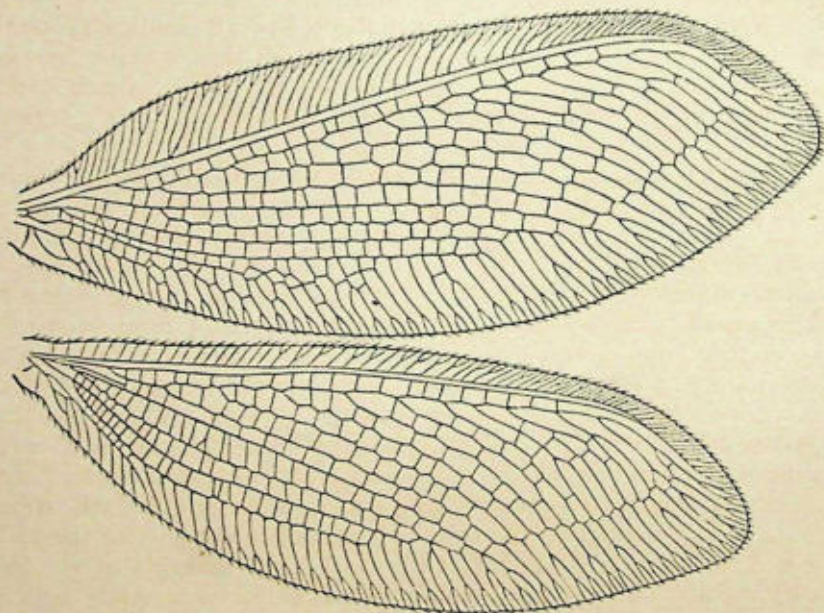
FIG. 4.—Wings of Parosmylus prominens , Ndm.
