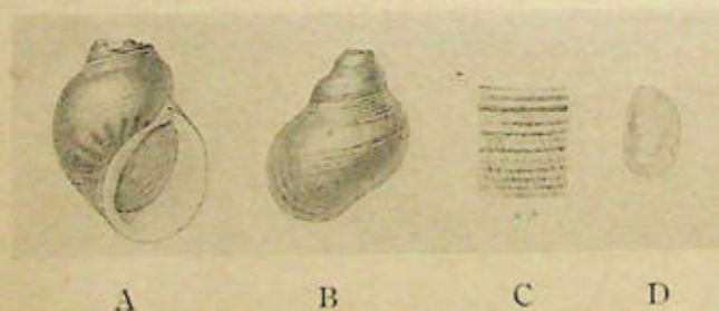
FIG. 1.—A, B, Paludomus annandalei , sp. nov.; C, Sculpture of same enlarged; D, operculum of same.
