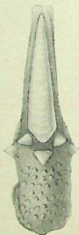
FIG. 2.— Scalpellum kamperi , \times 5 , back view.
