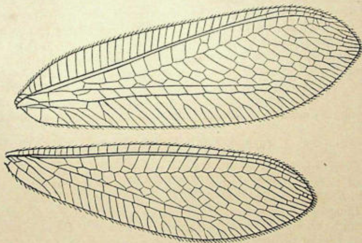
FIG. 3.—Wings of Tumeochrysa indica , Ndm.
