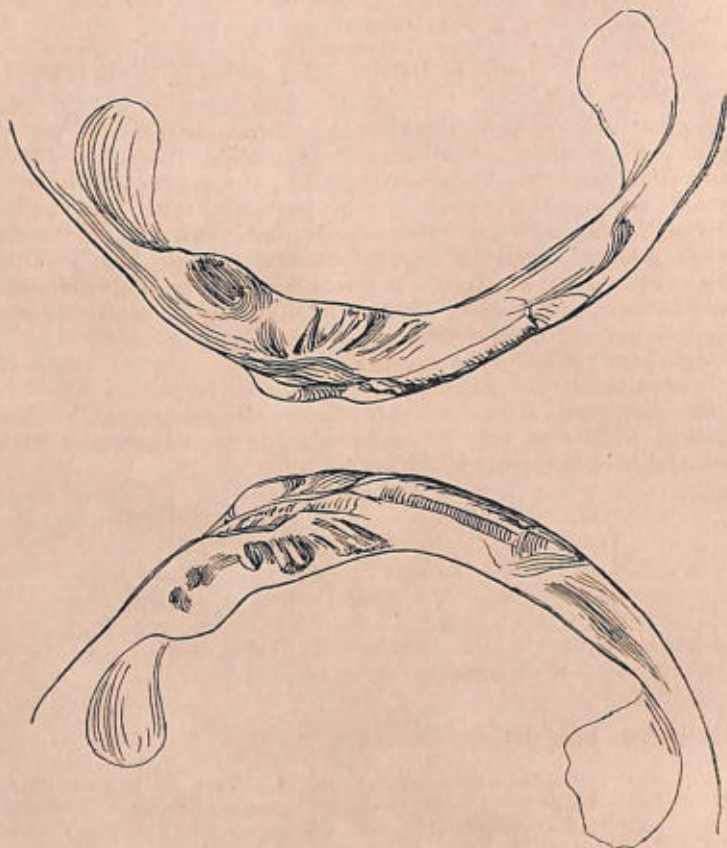
Fig. 26. — Cyrena impressa , Desh.; hinge of. Nat. size.
