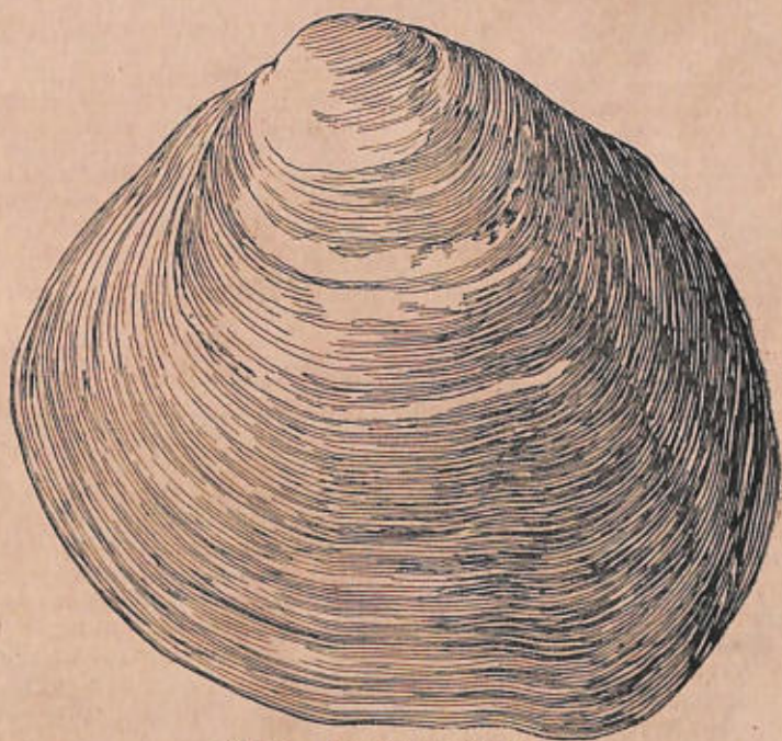
Fig. 25.— Cyrena impressa , Desh. (Type.) Nat. size.
