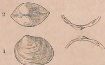
Fig. 28.— 1 & 2. Pisidium bombayanum , Theob. (Type.) \times 3 . 3. Hinge of the same. \times 3 .
