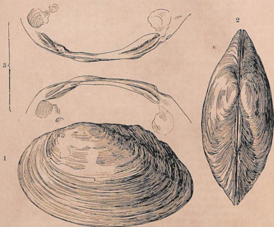
Fig. 16.—1 & 2. Parreysia ( P. ) daccaensis , Preston. (Type.) Nat. size. 3. Hinge and muscular scars of same.
