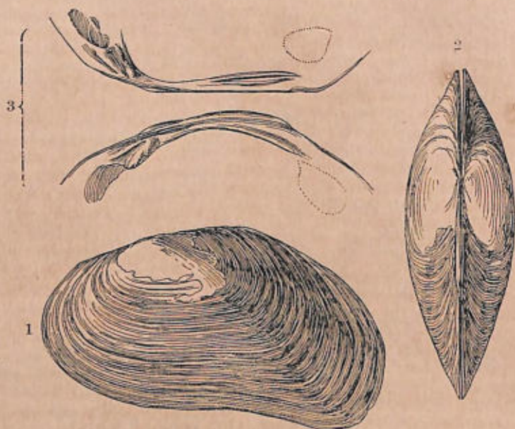
Fig. 8.—1 & 2. Nodularia (N.) theobaldi , Preston (type), nat. size. 3. Hinge and muscular scars of same.
