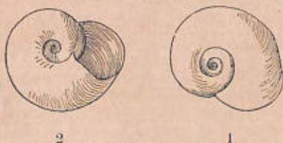
Fig. 5.— Planorbis (Gyraulus) labiatus , Bens. (Types.)
