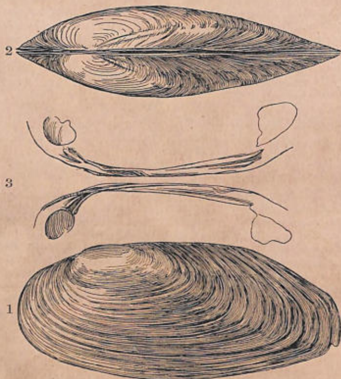
Fig. 21.—1 & 2. Lamellidens (L.) narainporensis , Preston. (Type.) Nat. size.
