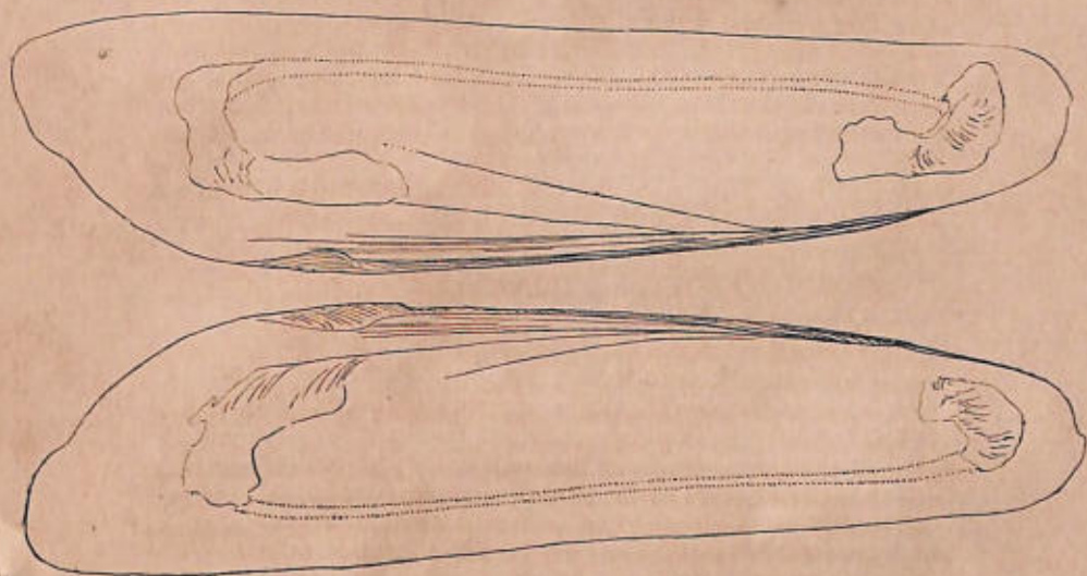
Fig. 6.— Solenaiia soleniformis (Benson) (specimen), nat. size, showing pallial line and muscular scars.
