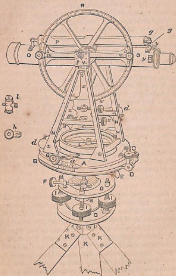
TRANSIT THEODOLITE.
