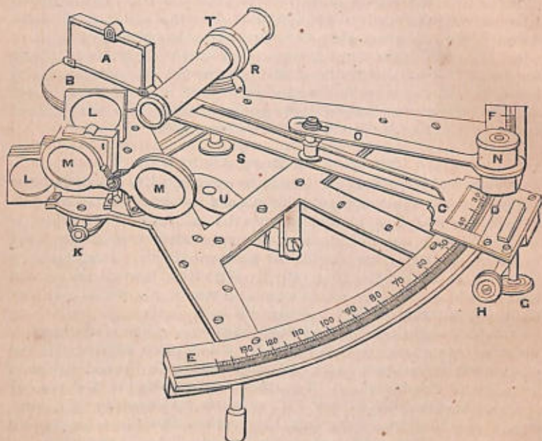
SEXTANT.
