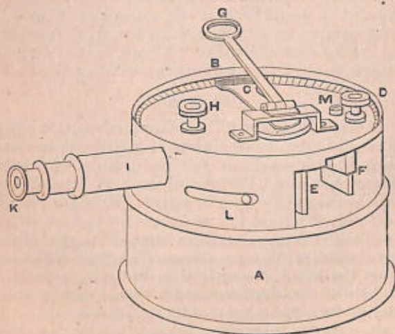
BOX SEXTANT.
