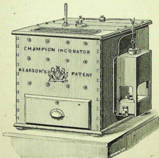
FIG. 12. HEARSON'S INCUBATOR.
