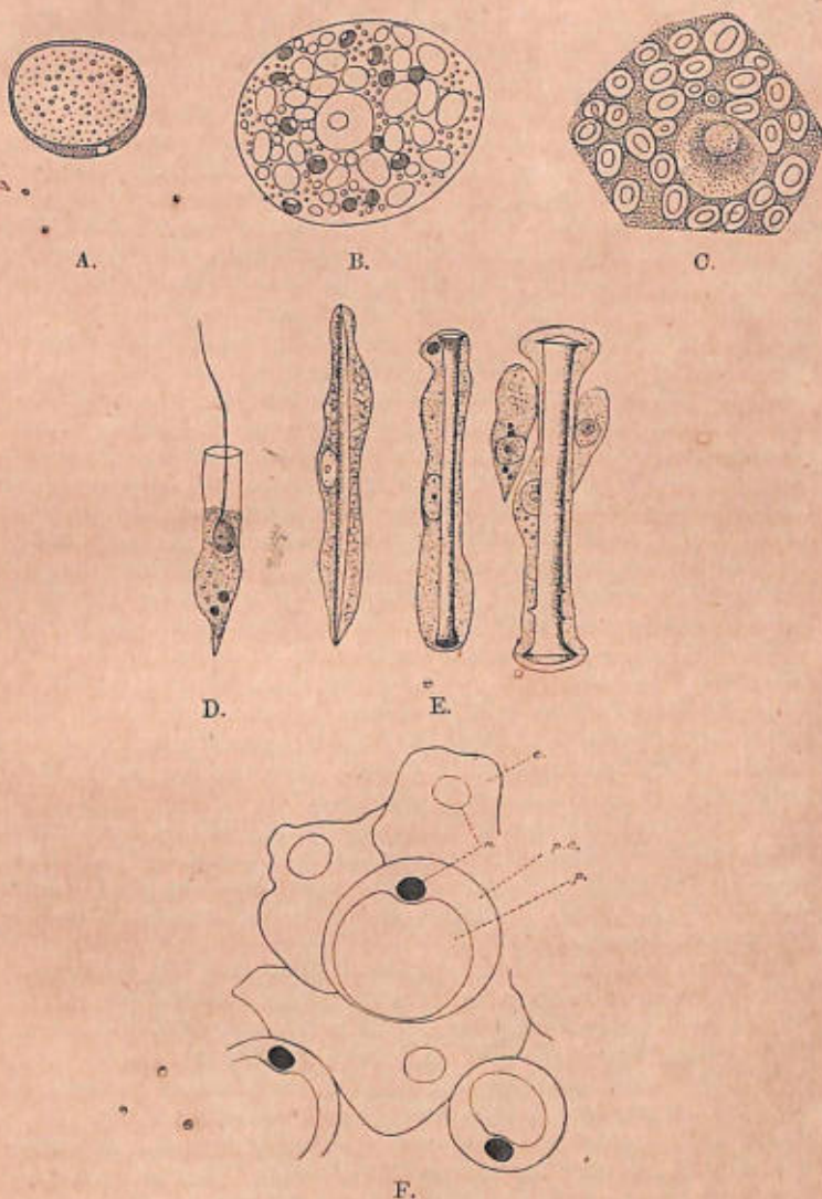
Fig. 2.—Sponge cells.
