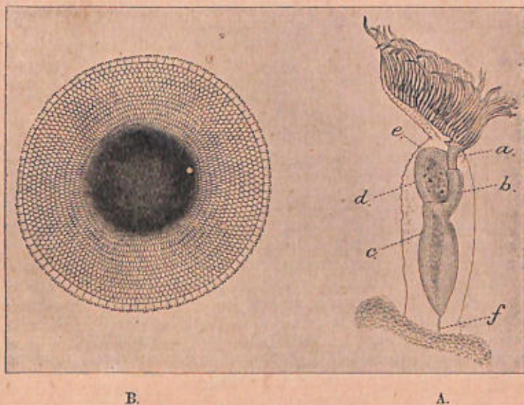
Fig. 47.— Pectinatella burmanica .
