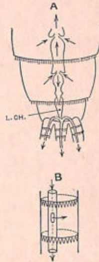
Fig. 571.—Hinder part of Nymph of a May-Fly ( Cloëon dipterum ), enlarged. A, Last three segments and bases of tail-rods. Last chamber (L.C.H.) of heart gives off vessels to the tail-rods. Arrows indicate direction of blood-flow. B, Part of a tail-rod, showing perforated walls of central blood-vessel.
