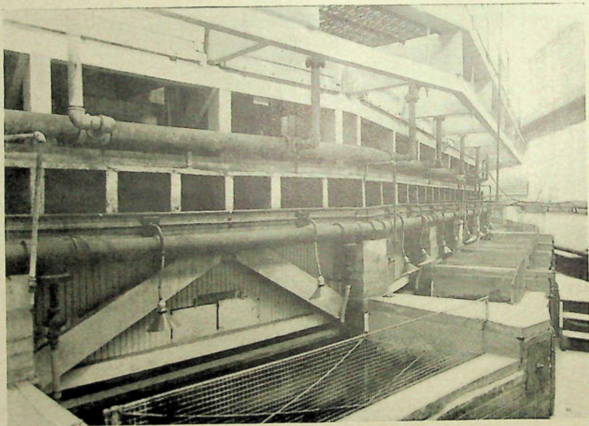
SERVICE GALLERY IN THE NEW YORK AQUARIUM. Showing the lower wall-tanks, reserve tanks, piping and electric lamps
