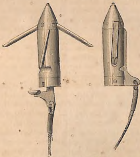
Fig. 16.—American Harpoon Ball.
