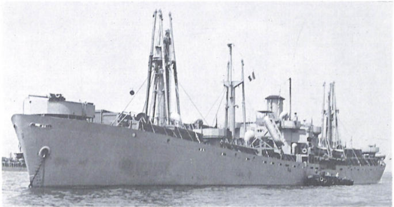
LIBERTY SHIP CLASS EC2-S-C1, FITTED FOR WAR SERVICE. Rigged model USNM 313022 shows the original design of the class. ( U.S. Maritime Administration photo 4423. )
