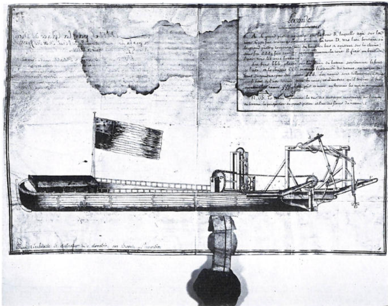
PATENT GRANTED TO JOHN FITCH BY LOUIS XVI OF FRANCE, November 29, 1791 (the original is in the Watercraft Collection USNM 130032). Propulsion is by "duck leg" paddles from the stern. The paddles are operated by cranks and pitman rods, driven by a chain, sprockets, and cranks from the steam engine. (Smithsonian photo 44795-a.)
