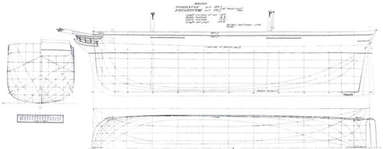
LINES OF THE NEW ENGLAND MERCHANT BRIGS Powhatan and Pocahontas , built at Newburyport, Massachusetts, 1829-30. An example of a model of burdensome freighting vessels favored in New England before the days of the clipper ships. Taken off the builder's half-model USNM 76060.
