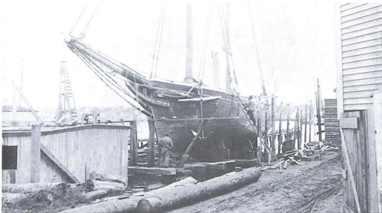
FISHING SCHOONER ON MARINE RAILWAY IN THE 1880's at Rocky Neck, Gloucester, showing the typical head work of an Essex-built fisherman of the period. ( Smithsonian photo 44791. )
