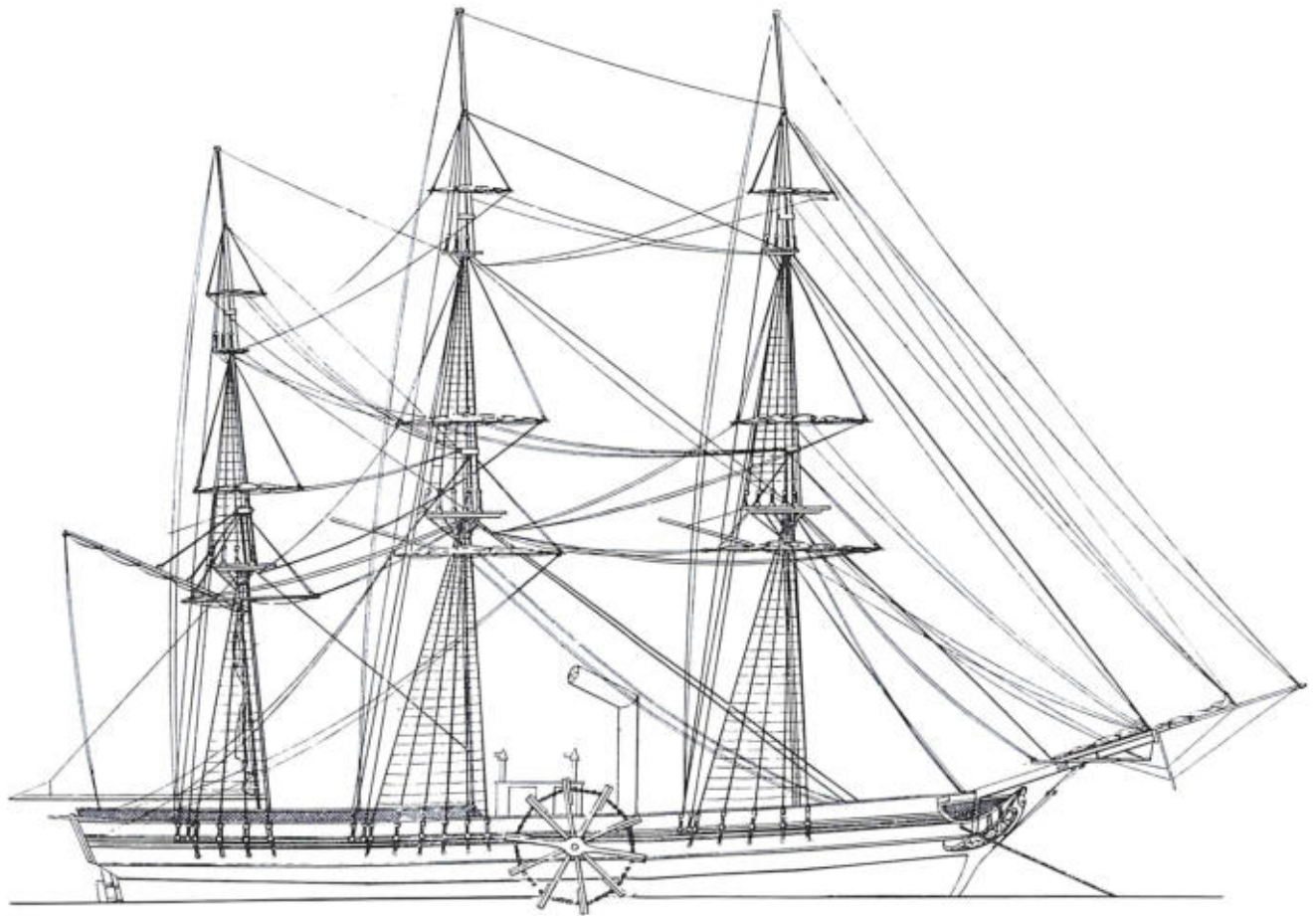
FIRST STEAMSHIP TO CROSS THE ATLANTIC, the Savannah , as drawn by the French naval constructor Marestier in 1820 and published in 1824 in his report on American steamers. (Smithsonian photo 45434-a.)
