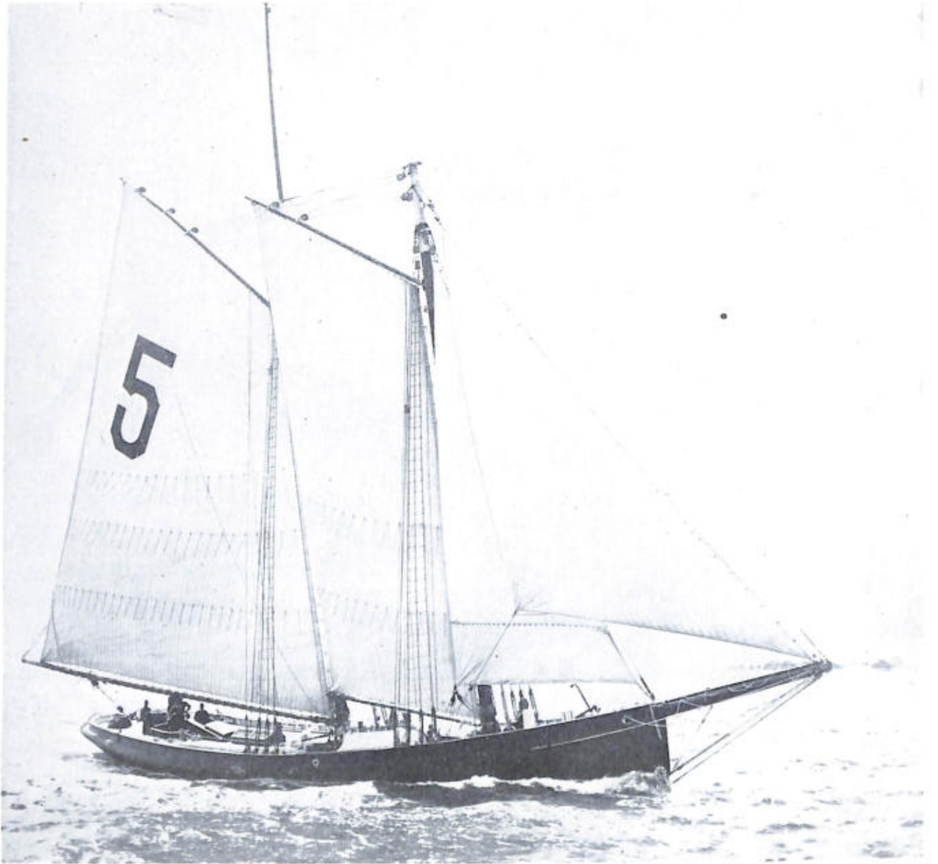
BOSTON PILOT SCHOONER Hesper , built at Chelsea, Massachusetts, by Dennison J. Lawlor, in 1884. Her register dimensions were 92' x 22' x 12', 98.94 gross tons. She is represented in the Watercraft Collection by the builder's half-model (USNM 76037; see p. 91). ( Smithsonian photo 37747-b. )
