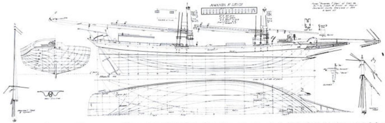
LINES AND DETAILS OF A CHESAPEAKE BAY PUNGY SCHOONER, the Amanda F. Lewis , built in 1884, one of the last of this now extinct type under sail. As taken off the vessel by the Historic American Merchant Marine Survey.
