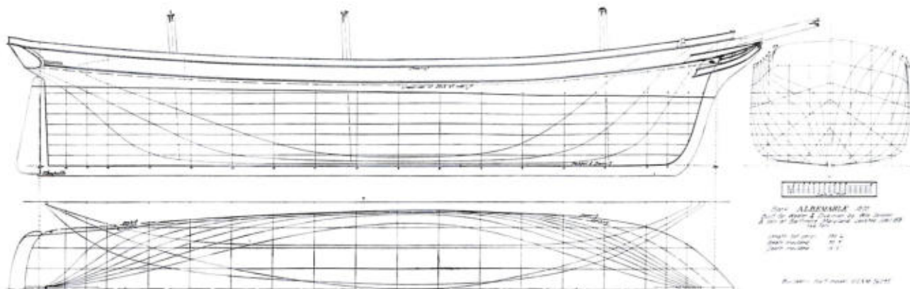
LINES OF THE COFFEE-CLIPPER BARK Albemarle , built at Baltimore, Maryland, in 1876. Taken off the builder's half-model USNM 76095.
