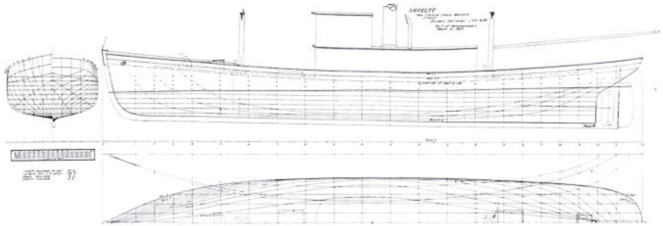
LINES OF THE STEAM MACKEREL SCHOONER Novelty , drawn from mould-loft drawing and checked with builder's half-model USNM 76286. In building, the foremast was placed 5 feet forward and the deckhouse was shortened, with the fore end and the stack 4 feet farther aft than shown.
