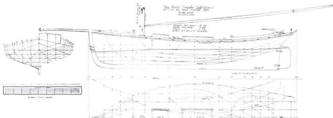
PLAN OF THE KEY WEST SMACKEE Jeff Brown built at Key West, Florida, 1883. Taken off the builder's half-model USNM 76086. Deck arrangement and spar dimensions from the rigged model USNM 76258.
