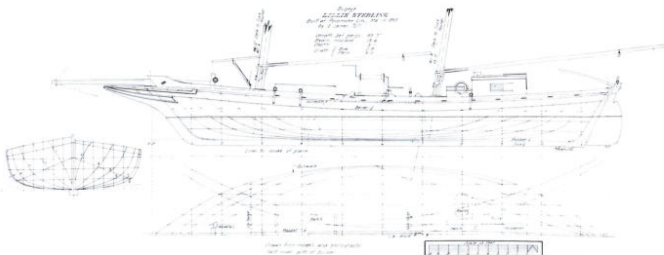
Lines of the small Chesapeake Bay bugeye, Lillie Sterling , built at Pocomoke City, Maryland, in 1885. The lines were taken off builder's half-model USNM 76290, the deck arrangement and spar dimensions are from rigged model USNM 76256.
