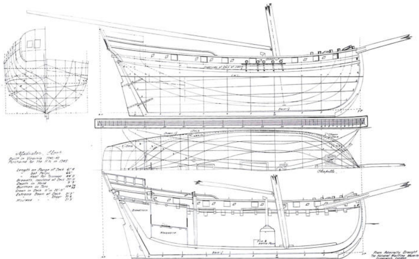
EARLIEST PLANS OF AN AMERICAN-BUILT VESSEL the sloop Mediator (see below), built on the Chesapeake, 1741-42. Redrawn from original British Admiralty draught. (Courtesy of Trustees of the National Maritime Museum, Greenwich, England.)
