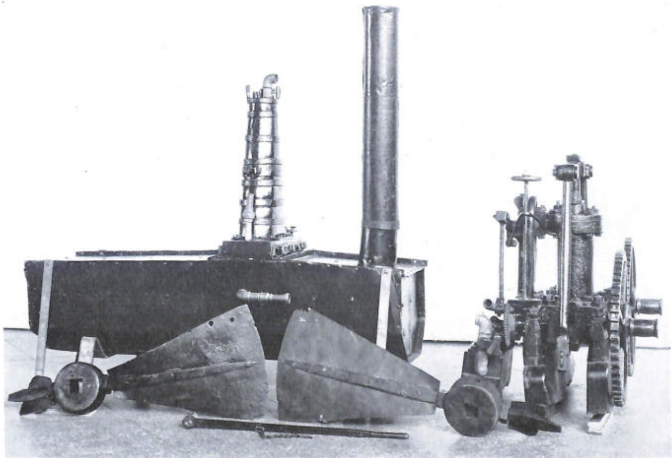
ENGINE AND BOILER (USNM 181179) DESIGNED BY JOHN STEVENS and used in his first steamboat, tested in New York Harbor, 1804. The propeller (USNM 180597) is a full-sized replica of the one used in tests in 1804-05. (Smithsonian photo 6151.)
