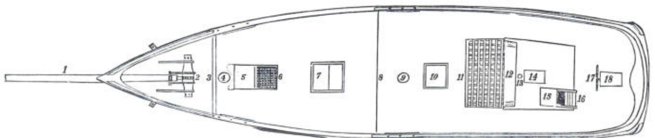
DECK PLAN OF MACKEREL SEINING SCHOONER of about 1885. From G. Brown Goode, The fisheries and fishery industries of the United States , Washington, Government Printing Office, 1884-87.
