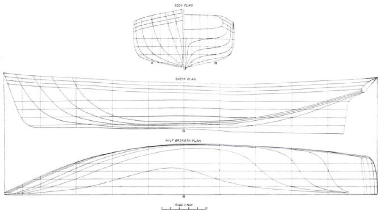
PLANS OF FISHING SCHOONER "MARY FERNALD."
