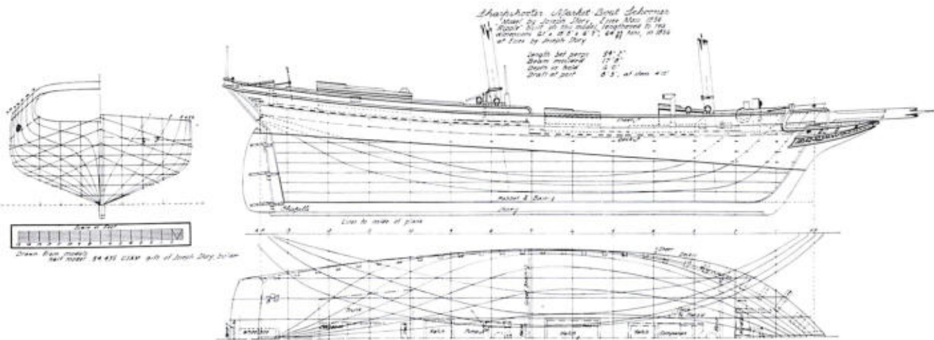
NEW ENGLAND SHARPSHOOTER MARKET-BOAT SCHOONER OF 1856. Taken off builder's half-model USNM 54435.
