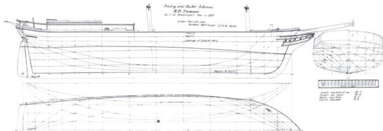
LINES OF THE COASTING AND PACKET SCHOONER R. B. Sumner , built at Newburyport, Massachusetts, in 1858. Taken off the builder's half-model USNM 76052.
