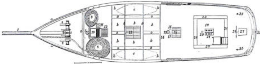
← INBOARD PROFILE AND DECK LAYOUT of a halibut-fishing schooner 1880, for fishing on Georges Bank. From G. Brown Goode, The fisheries and fishery industries of the United States , Washington, Government Printing Office, 1884-87.
