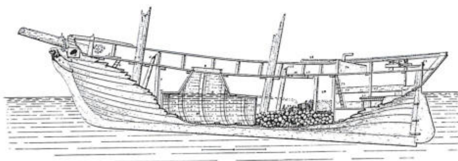
NEW ENGLAND WELL-SMACK for the fresh halibut fishery on Georges Bank, 1836-47. Longitudinal section, drawn by H. Elliott under the direction of Capt. J. W. Collins. From G. Brown Goode, The fisheries and fishery industries of the United States , Washington, Government Printing Office, 1884-87.
