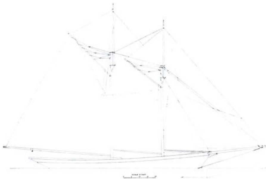
SAIL PLAN of the fishing schooner Fredonia , built in 1889, showing the spike bowsprit and small foresail then popular. From a probable copy of the plan of the designer Edward Burgess.
