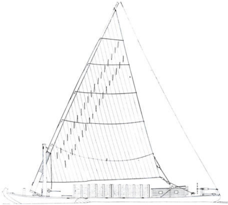
SAIL PLAN OF PISCATAQUA RIVER gundalow Fanny M. , showing rigging details. Drawn, under supervision of the builder of the gundalow, by the Historic American Merchant Marine Survey. (HAMMS 2-171-B.)
