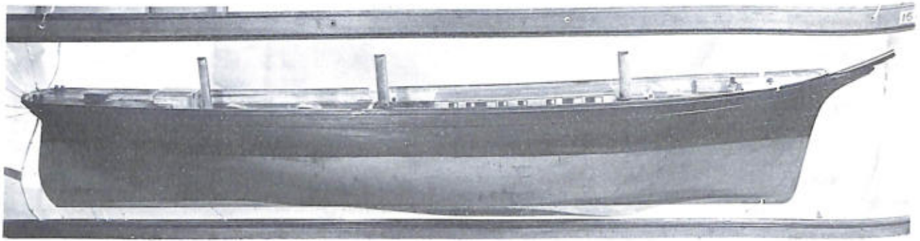
BUILDER'S HALF-MODEL OF CLIPPER SHIP MOUNTED AGAINST MIRROR TO SHOW DECK ARRANGEMENT. Young America , USNM 160135. (Smithsonian photo 20523.)
