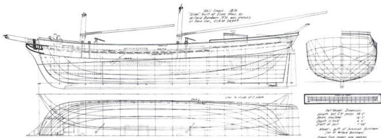
GLoucester Well-Smack, BUILT IN 1836, AT ESSEX, Massachusetts. Lines taken off the builder's half-model (USNM 54449) of the Glide .
