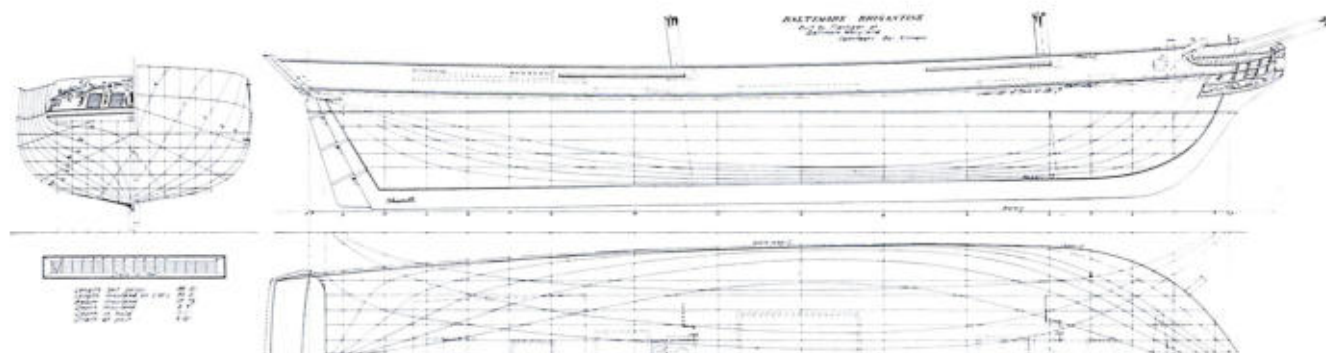
MERCHANT BRIGANTINE OF ABOUT 1818-28, BUILT AT BALTIMORE, MARYLAND, BY FLANNIGAN. Redrawn from a plan, by Hillman, formerly in the Webb Institute of Naval Architecture.
