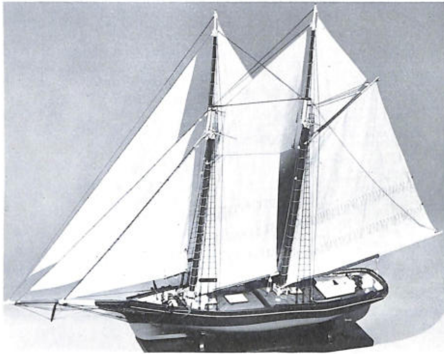
← FISHING SCHOONER Mary Fernald built at Gloucester, Massachusetts, in 1875 by Poland and Woodbury. She was designed by Daniel Pol- land, Jr. Rigged model USNM 76246. (Smithsonian photo 44693-k.)
