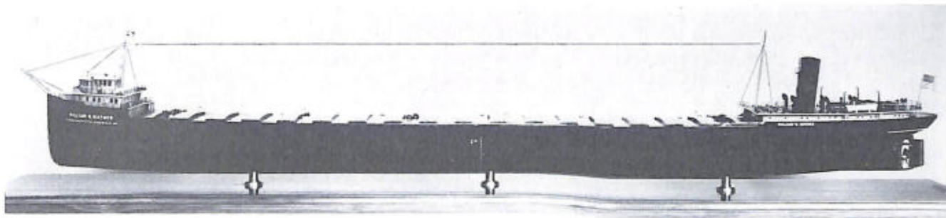
SINGLE-SCREW GREAT LAKES ORE AND BULK CARRIER William G. Mather , built at River Rouge, Michigan, in 1925. Rigger model USNM 312827. (Smithsonian photo 35710-b.)
