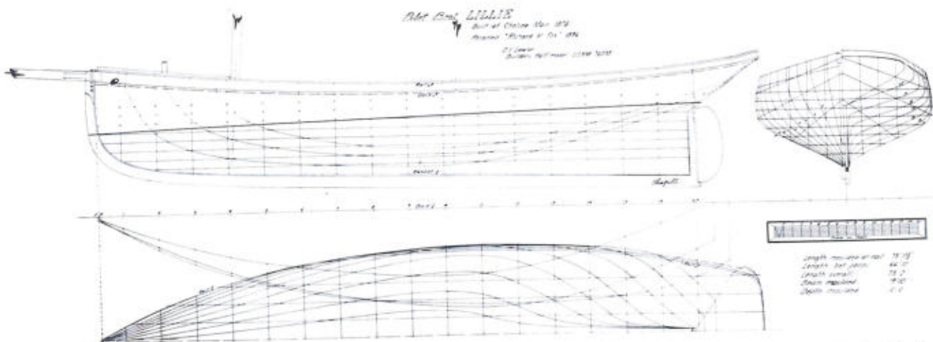
LINE OF THE BOSTON PILOT SCHOONER Lillie , built at Chelsea, Massachusetts, 1876. Taken off the builder's half-model USNM 76038.
