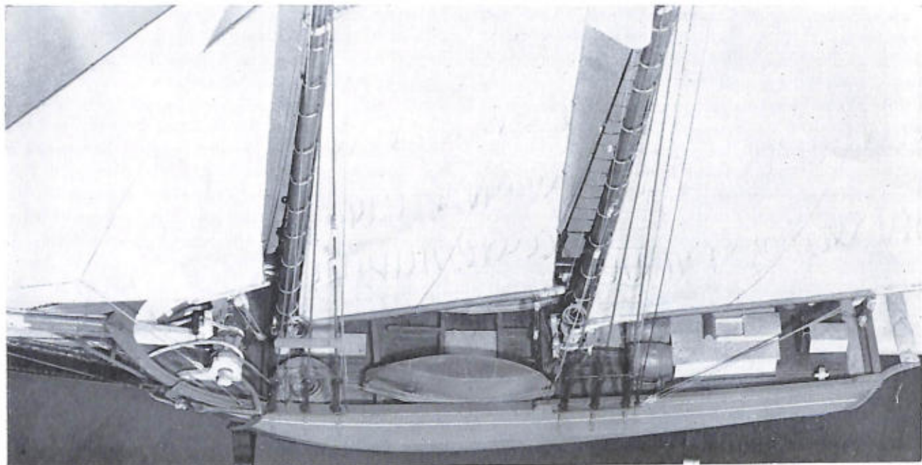
TYPICAL SHARPSHOOTER SCHOONER AT THE TIME THE SHARPSHOOTER WAS MERGING INTO THE CLIPPER MODEL. The Dauntless , built at Essex, Massachusetts, in 1855. Rigged model USNM 76244. Wooden stern davits for a yawl boat, and the standard deck arrangement of the period, can be seen. (Smithsonian photo 44695-a.)
