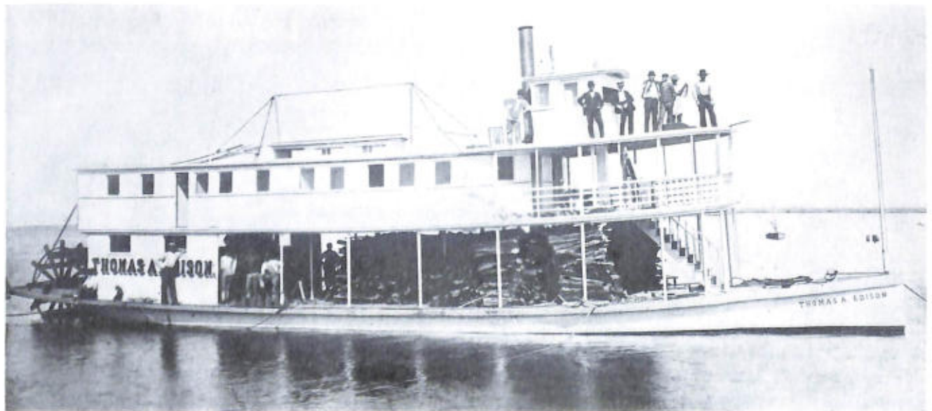
STERN-WHEEL RIVER STEAMER BUILT OF WOOD AT APALACHICOLA, FLORIDA, in 1901. The Thomas A. Edison is represented in the Watercraft Collection by builder's half-model USNM 311260. (Smithsonian photo 34432.)
