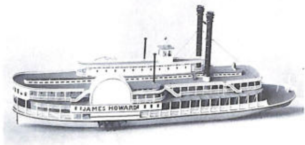
RIGGED MODEL (USNM 308426) of the Mississippi River packet steamer James Howard , built at Jeffersonville, Indiana, 1871, for the St. Louis to New Orleans run. (Smithsonian photo 30949-b.)
