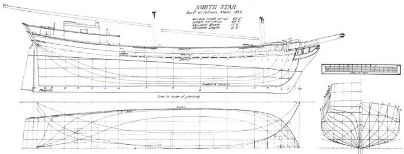
LINES OF THE 2-MASTED COASTING SCHOONER North Star , built at Sullivan, Maine, 1856. This vessel is somewhat similar to the early Marblehead type of fishing schooner. Taken off the builder's half-model USNM 76128.
