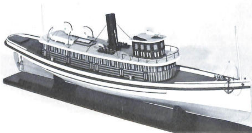
IRON STEAM TUG Rattler , built in 1879 at Philadelphia, Pennsylvania, by Neafie and Levy. This tug, was intended for coastwise towing. Rigged model USNM 160167. (Smithsonian photo 44693-d.)
