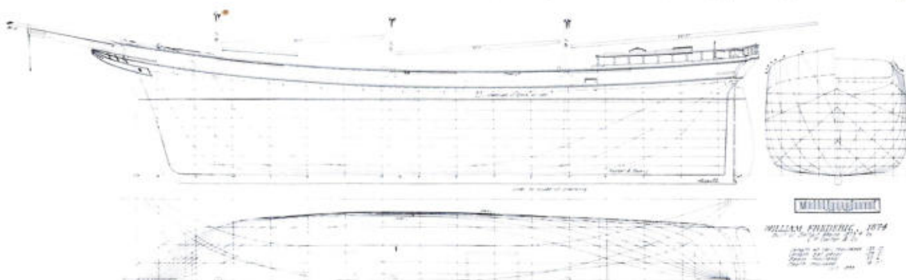
LINES OF THE 3-MASTED COASTING SCHOONER William F. Frederick , built, 1873-74, at Belfast, Maine, for the coastwise and West Indian trades. Taken off the builder's half-model USNM 76074.
