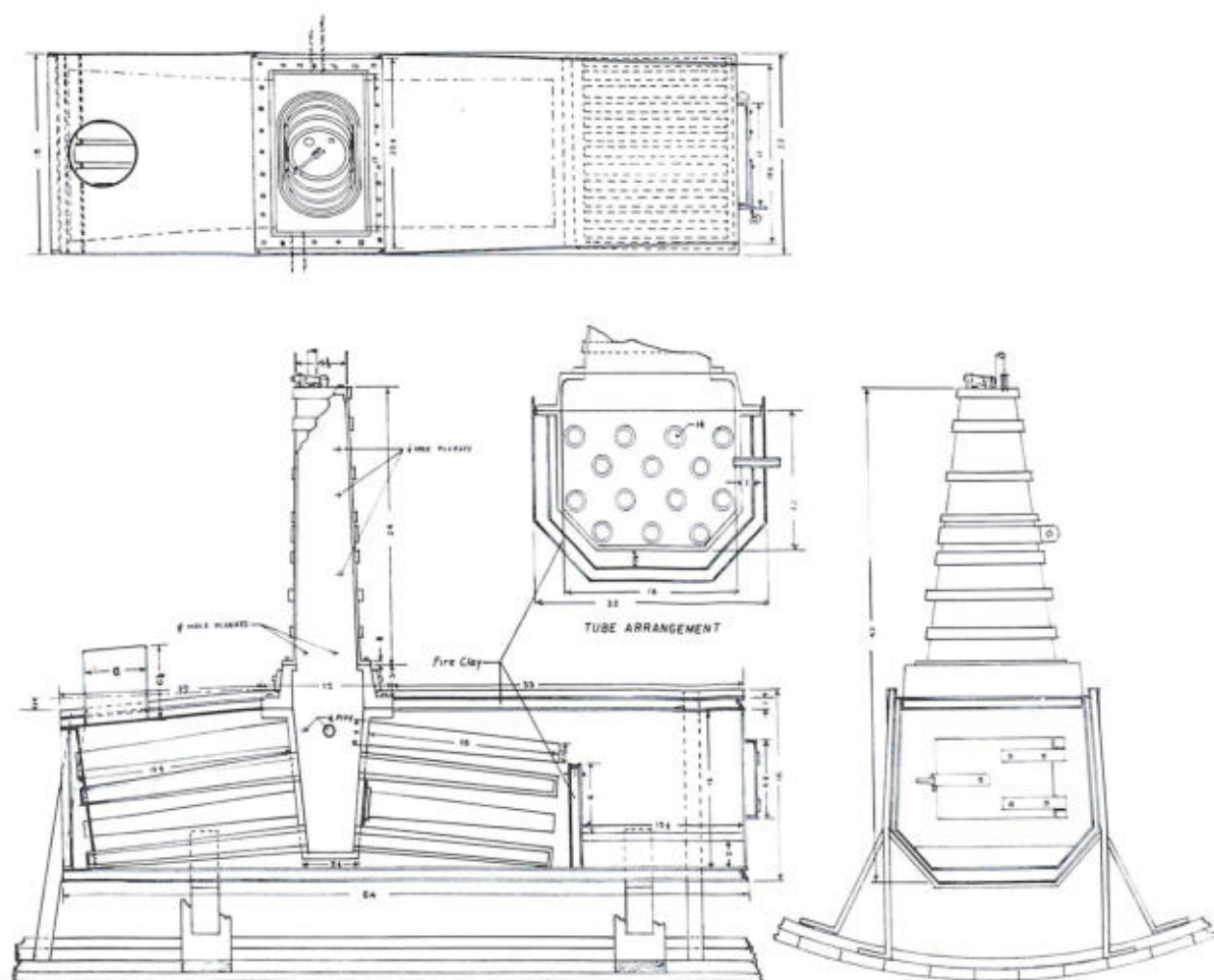
SCALE DRAWING OF MULTITUBULAR BOILER DESIGNED BY STEVENS and used by him in his steamboat, 1804. Original boiler (USNM 181179) is in the Watercraft Collection. (Smithsonian photo 45368.)
