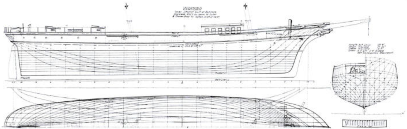
LINES OF THE LARGE 2-MASTED CLIPPER SCHOONER Vaquero , built as a packet at Baltimore, Maryland, 1852-53. Until lost at sea, she was employed in the Pacific between San Francisco, Melbourne, and Honolulu.
