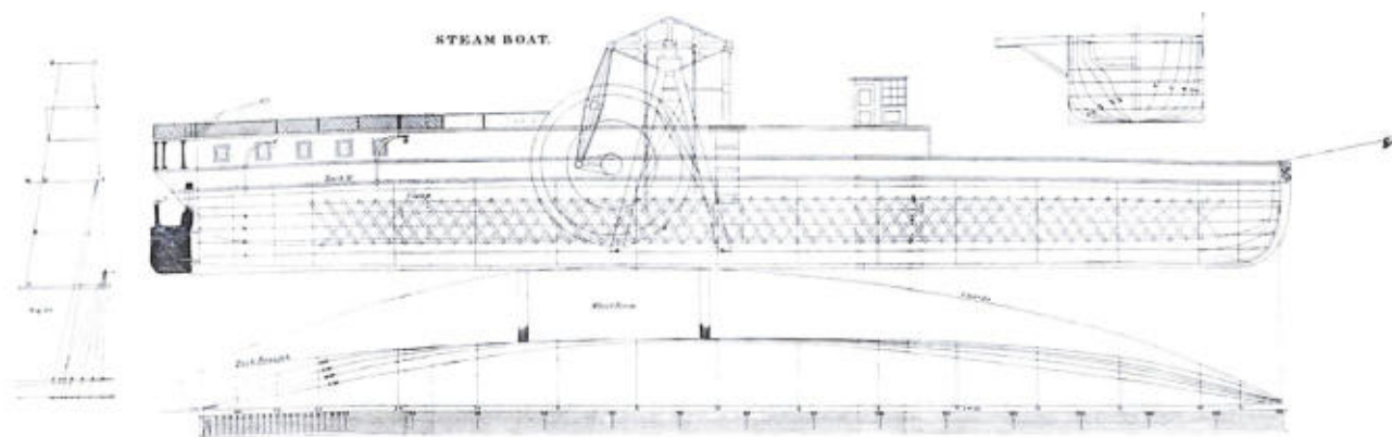
PLAN OF A SMALL HUDSON RIVER STEAMER OF ABOUT 1838, SHOWING DIAGONAL STRAPPING AND SHARP-ENDED FORM. After plate 7, in L. M'Kay, Practical shipbuilder , New York, 1838.
