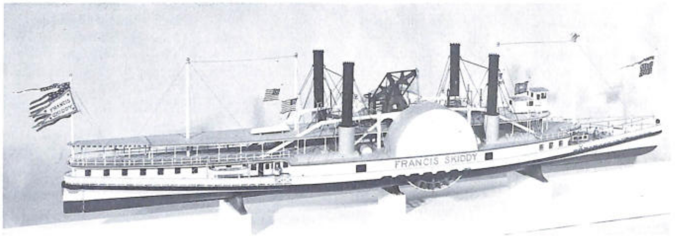
FAMOUS HUDSON RIVER STEAMER Francis Skiddy . Launched in 1849, she was capable of steaming 23-24 miles per hour. Wrecked in 1854. Rigged model USNM 316204. (Smithsonian photo 45666-h.)
