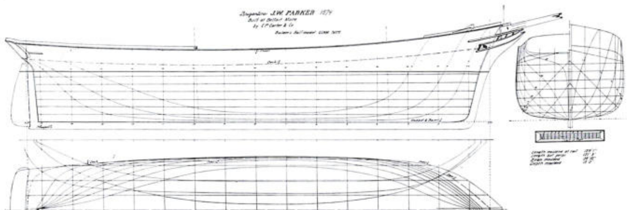
LINES OF THE BRIGANTINE, J. W. Parker , built at Belfast, Maine, in 1874. Taken off the builder's half-model, USNM 76075.
