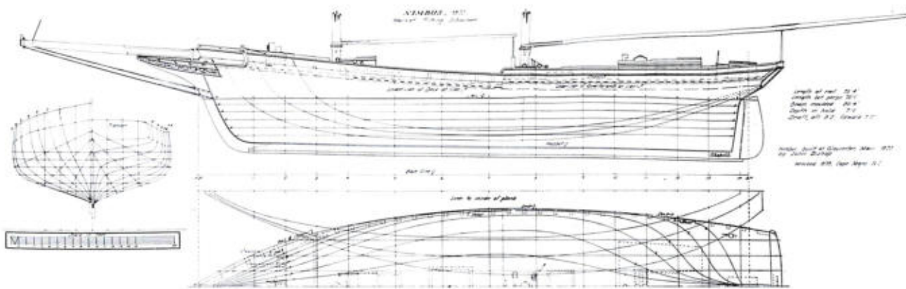
LINES OF EXTREME CLIPPER TYPE New England Fishing Schooner, the Nimbus , built at Gloucester, Massachusetts, in 1872. Taken off builder's half-model USNM 57052.
