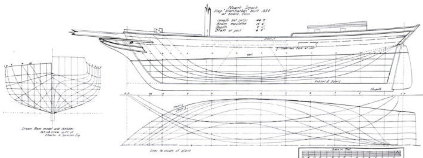
NOANK WELL-SMACK SLOOP Manhattan , built at Noank, Connecticut, in 1854 for the New York fisheries. Lines taken off builder's half-model USNM 160118.
