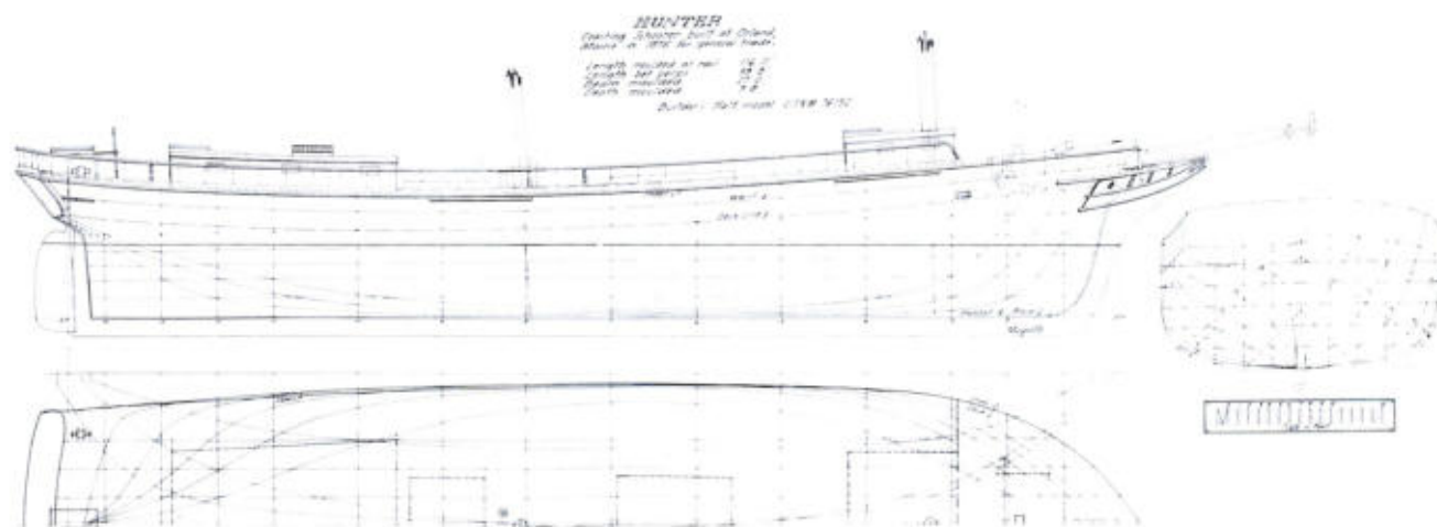
LINES OF THE LARGE, 2-MASTED COASTING SCHOONER Hunter , built at Orland, Maine, in 1876 for the general coasting trade. The plan shows a type popular in the early days of the coal trade. Taken off the builder's half-model USNM 76152.
