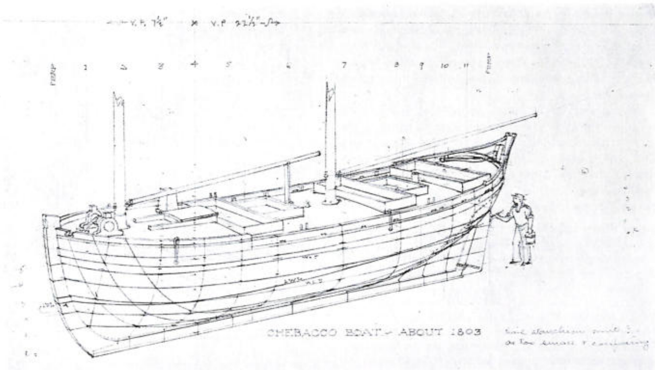
MEASURED PERSPECTIVE DRAWING OF A CHEBACCO BOAT, 1795-1805, showing form and arrangement of hull. Drawn by the late George C. Wales.
