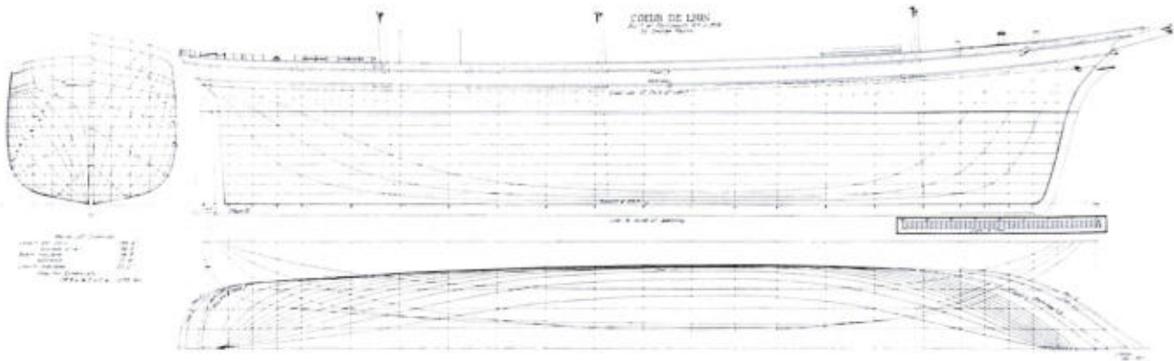
LINES OF THE MEDIUM CLIPPER Coeur de Lion built at Portsmouth, New Hampshire, in 1854. Taken off the half-model in the Portsmouth, New Hampshire, Athenaeum. A painting of this ship, in the Watercraft Collection, is shown, opposite.
