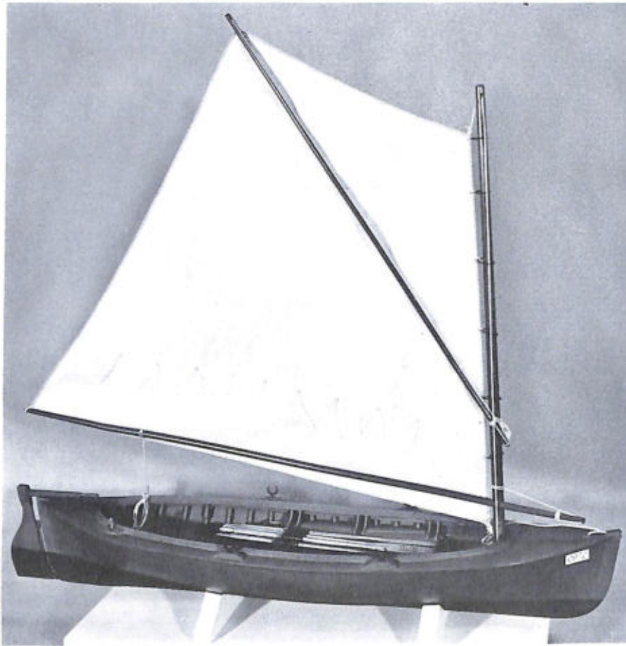
COLUMBIA RIVER SALMON BOAT of the type developed about 1885. Rigged model USNM 285033. (Smithsonian photo 45606.)
