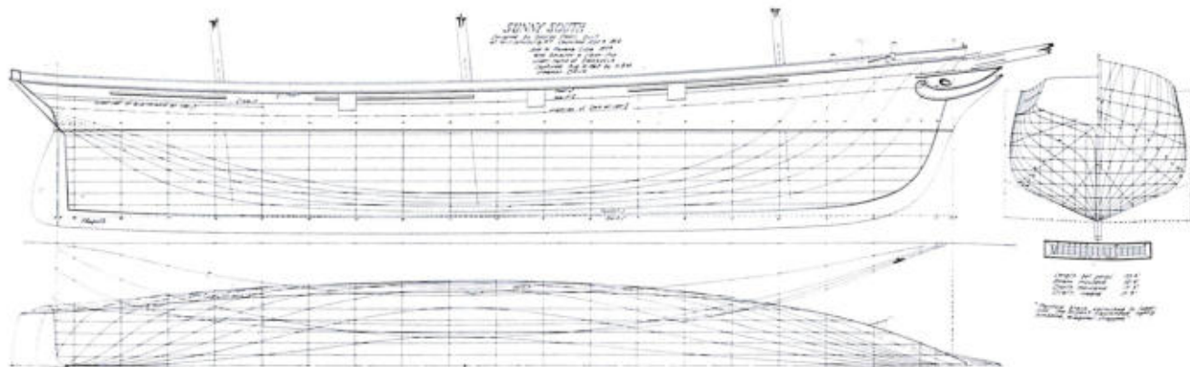
LINES OF THE EXTREME CLIPPER Sunny South , built at Williamsburg, New York, in 1854. She became the slaver Emanuela . Taken off the half-model in the Mariners' Museum, Newport News, Virginia.
