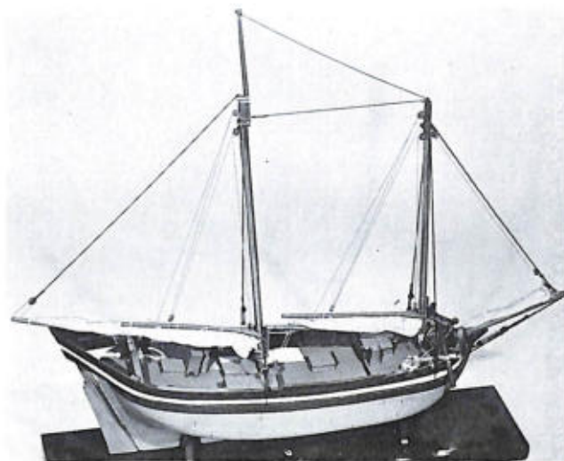
NEW ENGLAND PINKY of 1820-45, rigged model USNM 57586, showing a typical deck arrangement. The mainsheet horse forward of the tiller, however, is unusual and probably an error of the model builder. (Smithsonian photo 44694.)
