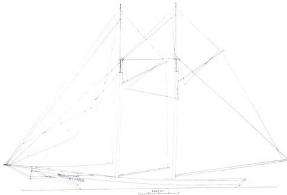
← SAIL PLAN of the fishing schooner Mary Fernald , from a copy of the sailmaker's plans in the Watercraft Collection.
