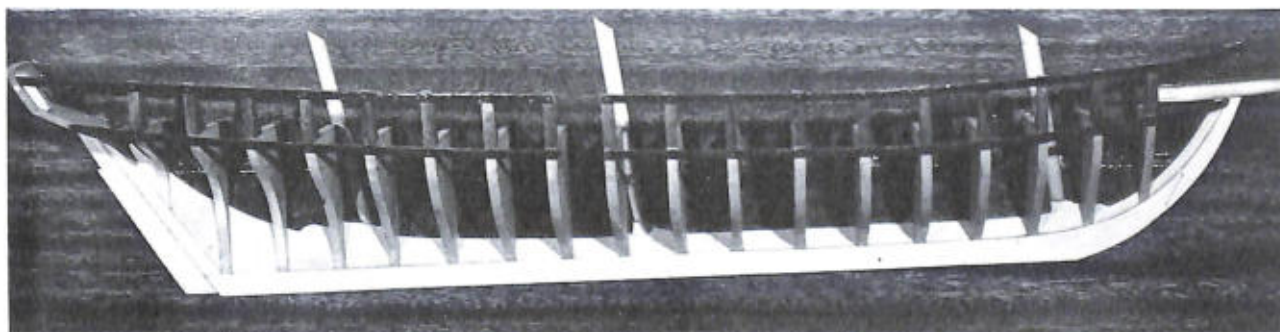
HAWK'S NEST, OR CROW'S NEST, HALF-MODEL, WITH KEEL AND DEADWOOD FORM SHOWN. Mould-sections were at alternate frames, and sheer and deck lines were indicated by the use of battens tacked to moulds. The keel detail shown is unusual. One of the older forms of builder's half-models, this one, in the author's collection, is of the 3-masted Baltimore schooner Flying Fish of about 1806. (Smithsonian photo 45607-c.)
