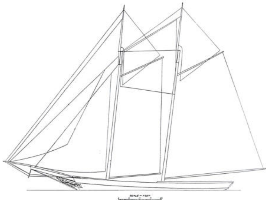
SAIL PLAN FOR A GRAND BANKER BUILT AT ESSEX, MASSACHUSETTS, IN 1859, the Break O' Day . From a copy of the sailmaker's plan in the Watercraft Collection.
