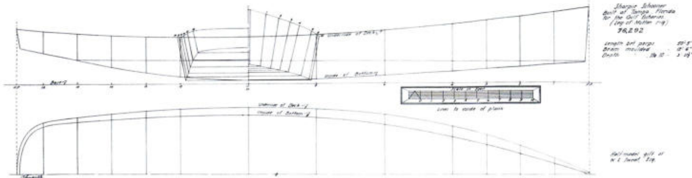
LINES OF A FLORIDA SHARPIE SCHOONER, BUILT AT TAMPA, FLORIDA, about 1891-92. Taken off builder's half-model USNM 76292.
