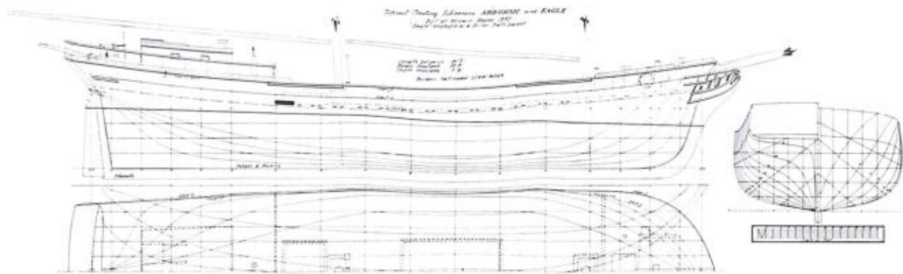
LINES OF THE SQUARE-TOPSAIL COASTING SCHOONERS Arrowsic and Eagle , built at Arrowsic Island, Kennebec River, Maine, in 1847. The Eagle was employed as a New York to Bath packet. Taken off the builder's half-model USNM 76069.
