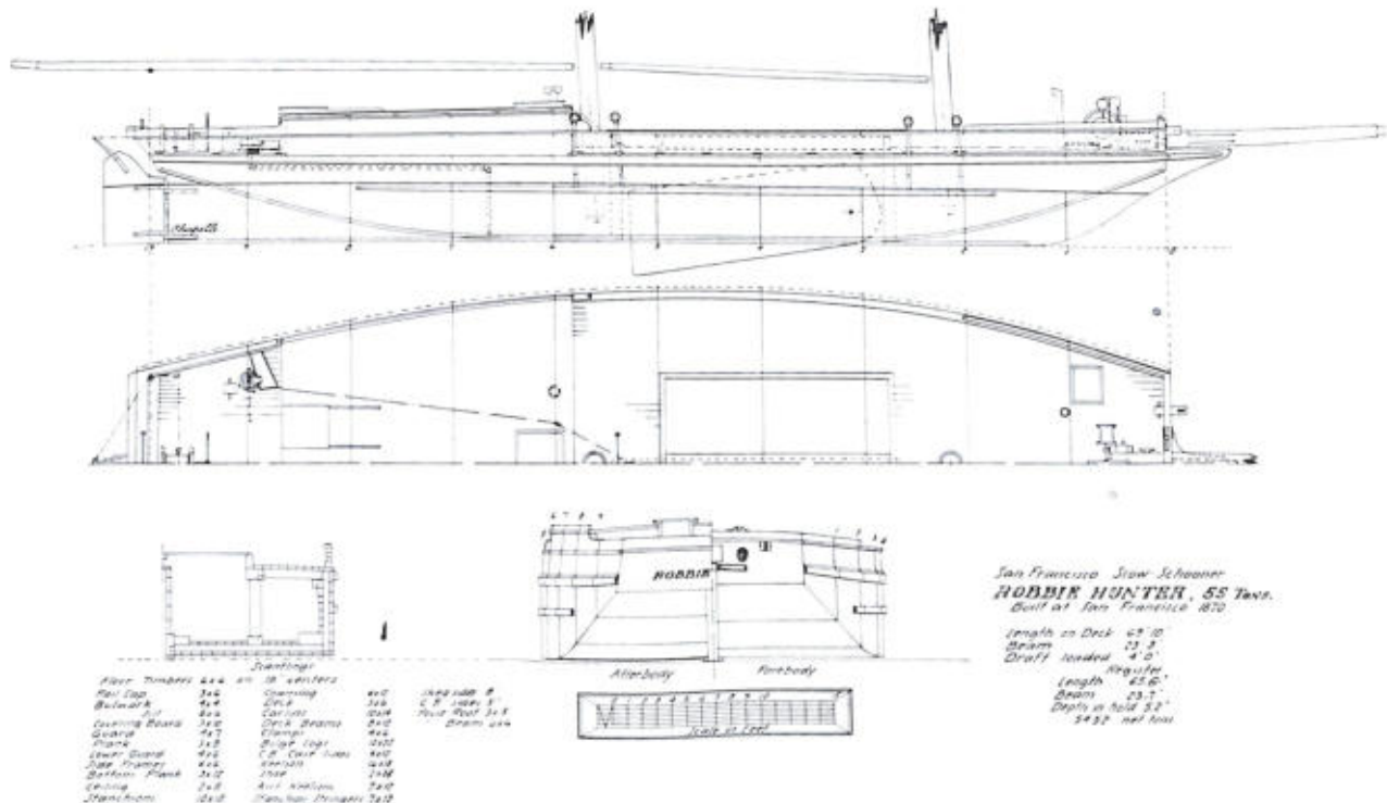
LINES OF SAN FRANCISCO 2-MASTED SCOW SCHOONER Robbie Hunter , built in 1870. As taken off by the Historic American Merchant Marine Survey.
