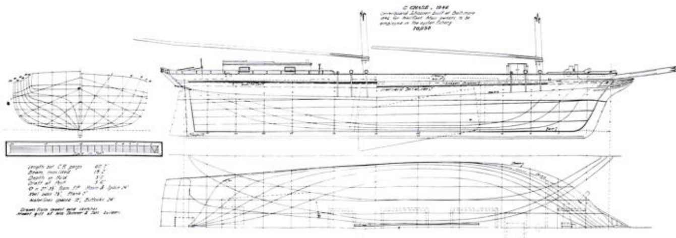
CENTERBOARD FISHING SCHOONER, about 1846 BUILDER'S HALF-MODEL, USNM 76098
