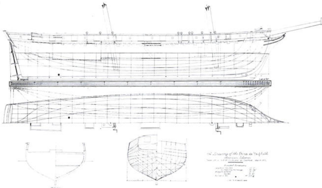
PLAN OF A PRIVATEER BUILT BY ADAM AND NOAH BROWN, NEW YORK, DURING THE WAR OF 1812. The Prince de Neufchatel , after a successful career as a privateer, was captured by the British and plans were made of her. She was noted for her speed, and was probably similar to the General Armstrong . Redrawn from the original British Admiralty draught.
