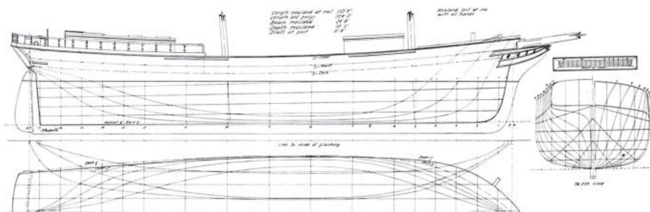
Lines of the Baltimore-built brigantines George Latimer and Alexander Kirkland , built 1858 for the West Indian trade. The Latimer was destroyed by the Confederate cruiser Florida , and the Kirkland disappeared at sea. Taken off builder's half-model USNM 76099.
