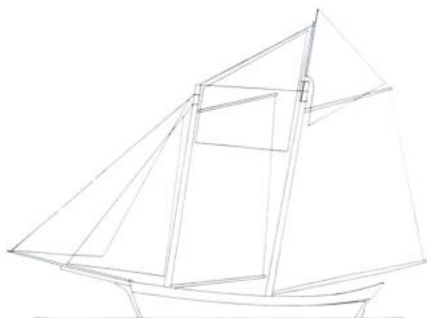
TYPICAL PINKY SAIL PLAN, FOR THE PERIOD 1824-45, of the Lorenzo D. Story , of about 1842.
