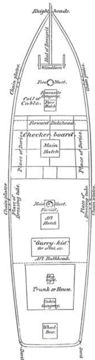
Sketch of the Deck of COD SCHOONER Centennial , Capt. B.A. Williams, Gloucester, Mass.
