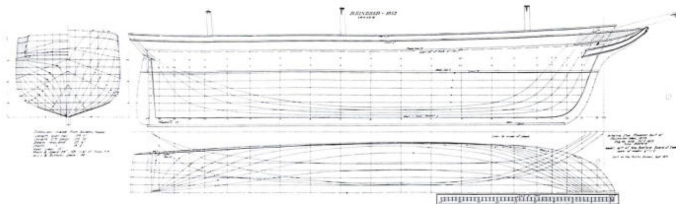
LINES OF WHALING SHIP BUILT AT ROCHESTER, MASSACHUSETTS, IN 1853. The Reindeer is an excellent example of the clipper-model whalers built for the Bering Sea whale fishery in the 1850's. Lines taken off builder's half-model USNM 160124.
