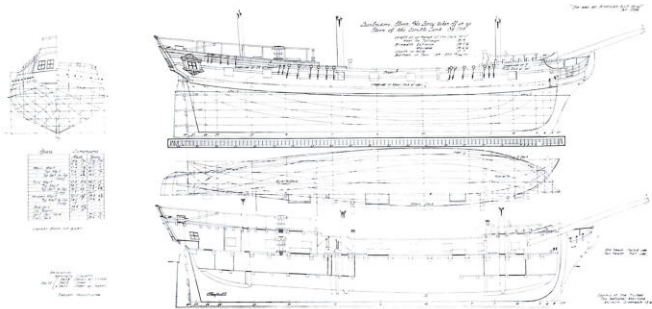
AMERICAN PRIVATEER SHIP OF THE REVOLUTION, ORIGINAL NAME UNKNOWN, taken into the British Navy in 1784 as the Barbadoes . This plan, redrawn from original British Admiralty draught, shows an early "sharp-model" vessel built for fast sailing, one of the ancestors of the clipper ship. (Courtesy of Trustees of the National Maritime Museum, Greenwich, England.)
