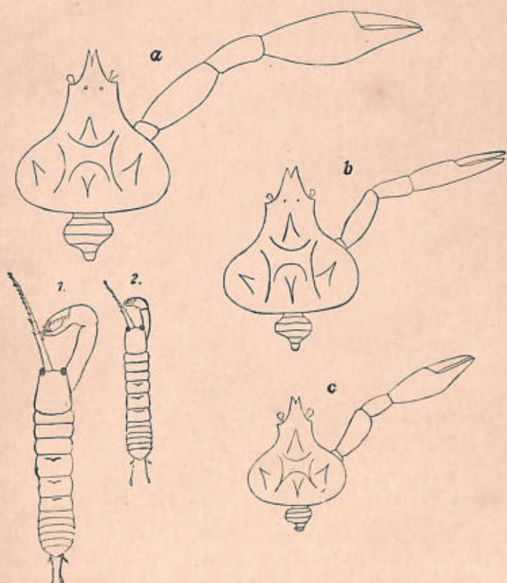
FIG. 95.—1, 2, two male forms ("high" and "low") of Leptochelia dubia . a, b, and c, the three male types of Inachus thoracicus (high, middle, and low).
