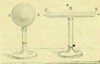
Fig. 69. — Electrifying action. — The vicinity of the ball A, charged with positive electricity, brings into C a negative electricity, and at D positive electricity.
