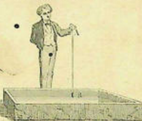
Fig. 97. — Vertical line AB is perpendicular to the surface of the water.
