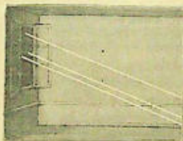
Fig. 25. — Light travels in a straight line.
