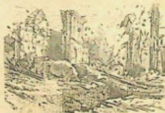
Fig. 31. — Earthquake.
