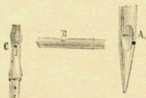
Fig. 53. — A, orifice of the pipe of an organ. — B, of a flute. — C, of a flageolet.
