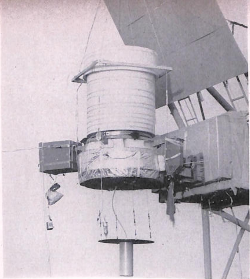
Smithsonian-built gamma-ray detector is a spark chamber connected to a closed-circuit television system, by which a spark pattern can be registered and telemetered back to earth. Launched from Flight Station of the National Center for Atmospheric Research at Palestine, Texas, May 28, 1966, it was carried 120,000 feet aloft in an 8½-hour flight. Data analysis is underway.
