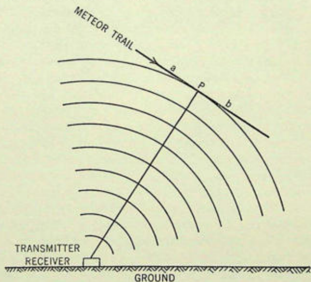
FIGURE 9.—Schematic diagram showing the geometry of radio echoes reflected from the ionization trail of a meteor.
