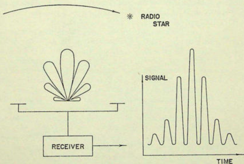
FIGURE 2.—A radio interferometer and the signal it produces when a radio star passes through the antenna pattern.
