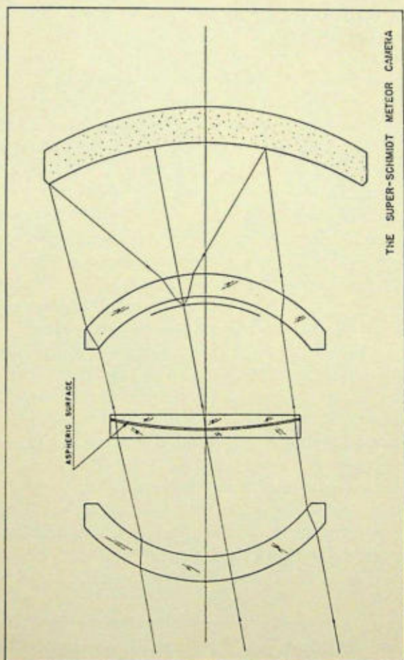
FIGURE 4.—Design of the optics of the Baker Super-Schmidt meteor camera.
