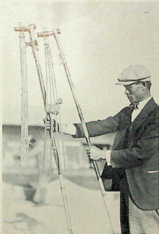
2. Flexible and resilient bamboo, grown on the place, provides the Oriental farmer the wherewithal to make his own threshing machine. Obihiro, Japan.
