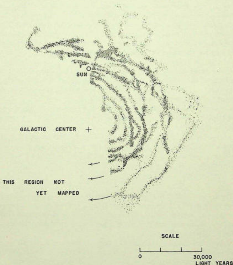
FIGURE 4.—Spiral structure of the local galaxy. (Reproduced by permission of G. Westerhout and M. Schmidt, Leiden, Holland.)
