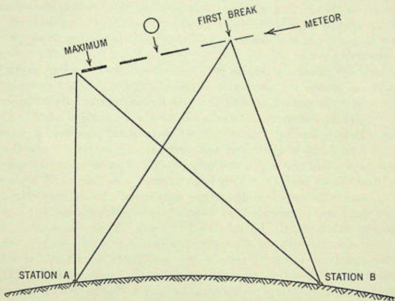
FIGURE 3.—Diagram showing a meteor photographed simultaneously from stations A and B; the circle represents a common point on both photographs of the trail.
