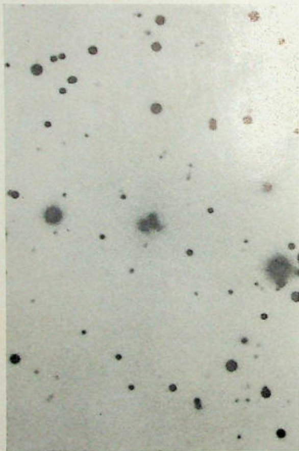
1. Galaxies in collision. (Photograph by permission of Mount Wilson and Palomar Observatories.)
