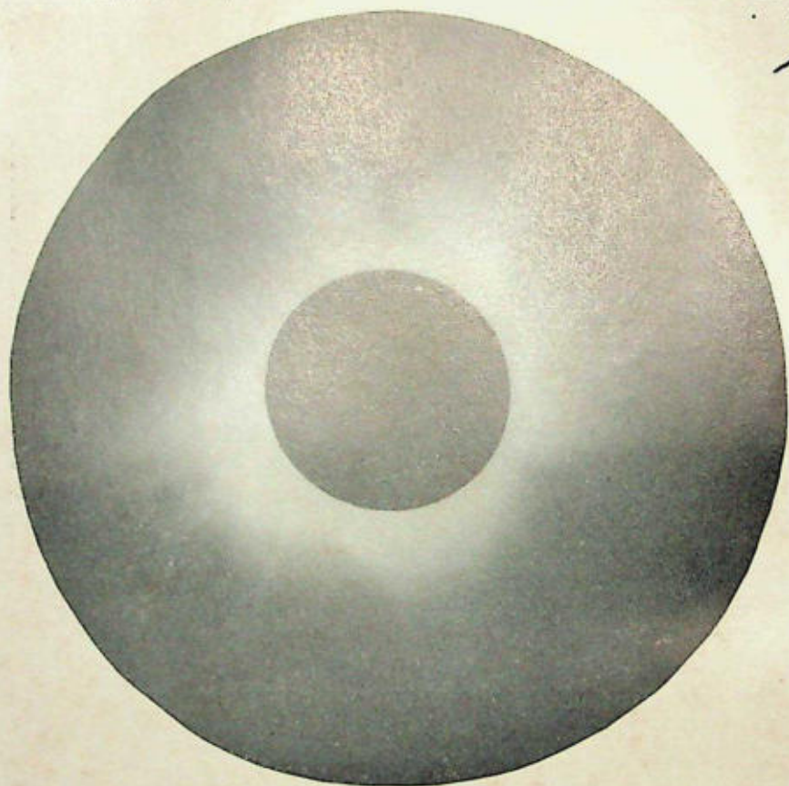
The solar corona photographed by Harvard during the 1937 solar eclipse.
