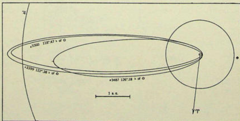
FIGURE 7.—The orbits of three \delta -Aquarid meteors ( q=0.07 A. U.)
