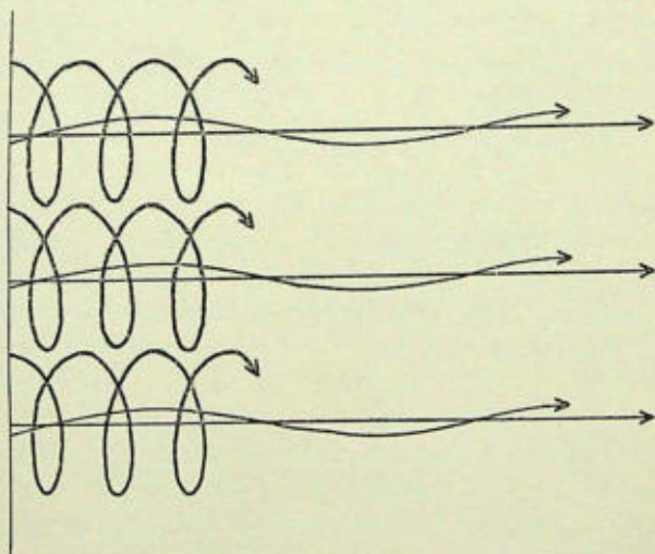
FIGURE 1.—Diagram illustrating how particles that embarked on spiral orbits of different pitch will be delayed differently and why late arrivals will appear to come from a variety of directions different from the main direction. The size of the earth is small compared with the radius of the spirals.
