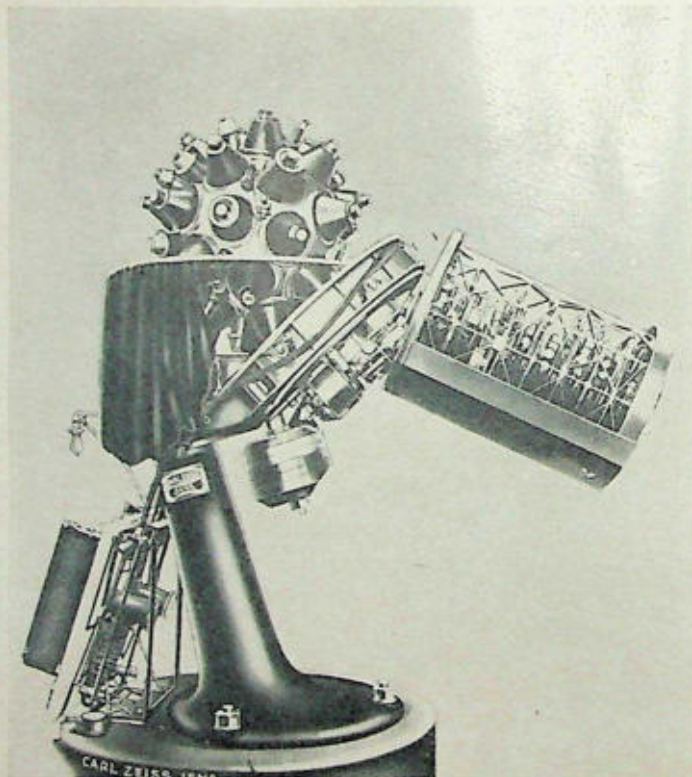
1. Projection apparatus of the Carl Zeiss Jena Planetarium.
