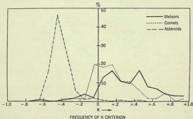
FIGURE 5.—The frequency of the criterion K among meteors, comets, and asteroids.
