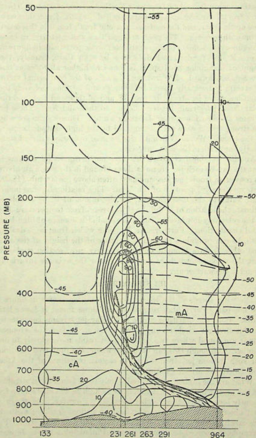
FIGURE 2.—View of continental-arctic jet stream seen looking downwind (after McIntyre and Lee, 1954). Lower numbers identify Alaskan and Yukon stations. Ordinate is pressure in mb. Solid lines are isotachs in knots. Broken lines are isotherms in °C. Heavy solid lines show frontal surface and tropopause.
