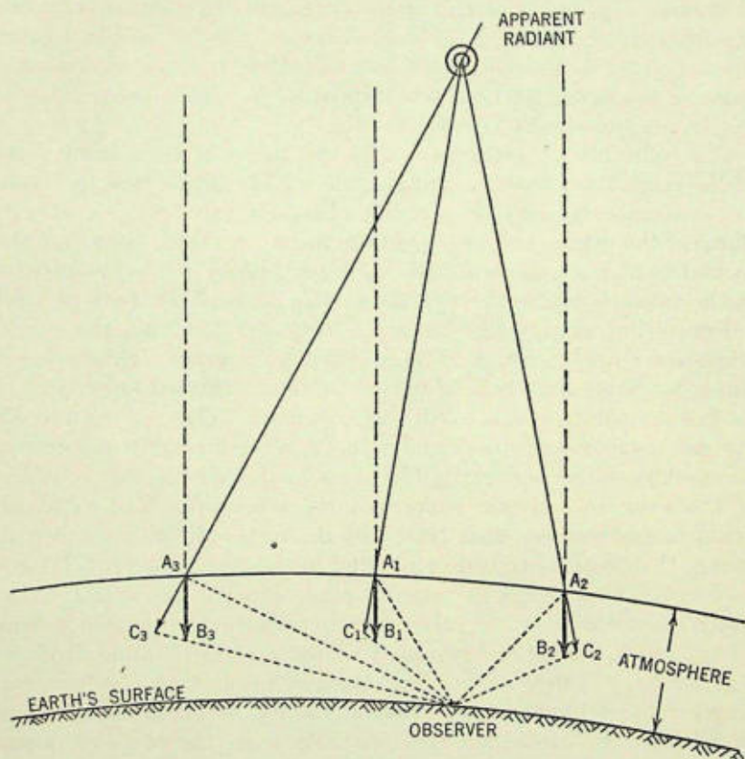
FIGURE 2.—Trails and radiant of a meteor shower. Above the atmosphere the parallel dashed lines show the real paths of the meteors A_1 , A_2 , and A_3 ; solid lines show their apparent paths. In the atmosphere the arrows AB show the real meteor paths, and the arrows AC show the paths as they appear to the observer.
