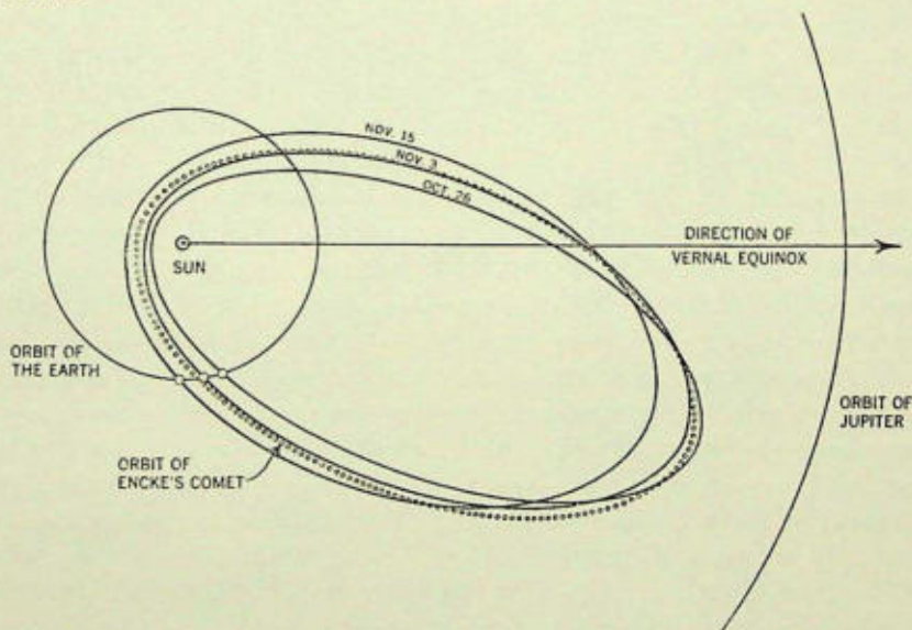
FIGURE 8.—The orbits of Encke's comet, and of three meteors of the associated northern Taurid shower that struck the earth's atmosphere on the dates shown.
