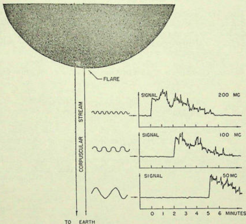
FIGURE 3.—Radio signals produced by a corpuscular stream as it travels through the atmosphere of the sun. (Photograph taken at the Astrophysical Observatory, Kodaikanal, India.)
