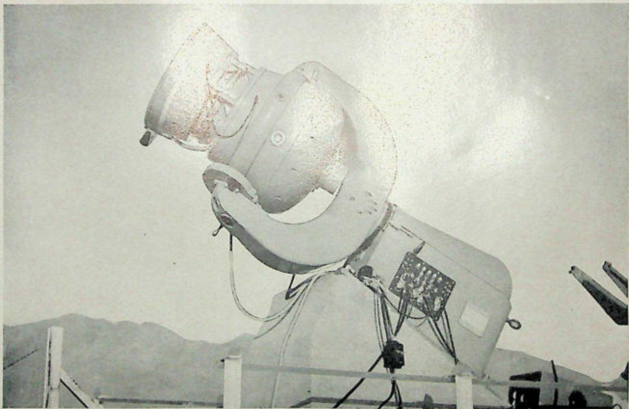
The Baker Super-Schmidt meteor camera.
