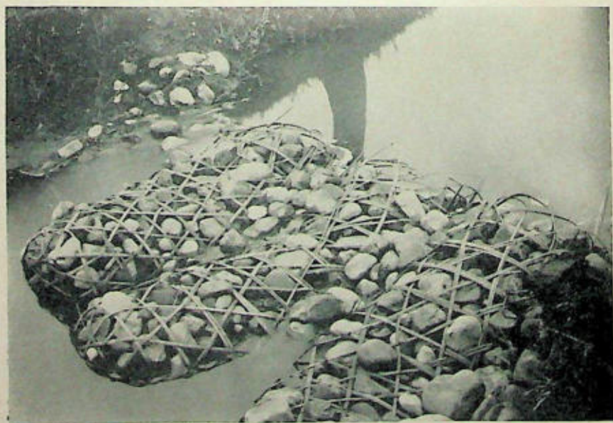
2. Although the bamboo withes from which they are made appear frail and inconsequential, these baskets effectively stabilize a footbridge of field stones near Kao-dien, Hupeh Province, China. (Photograph by F. N. Meyer, from the U. S. Department of Agriculture.)
