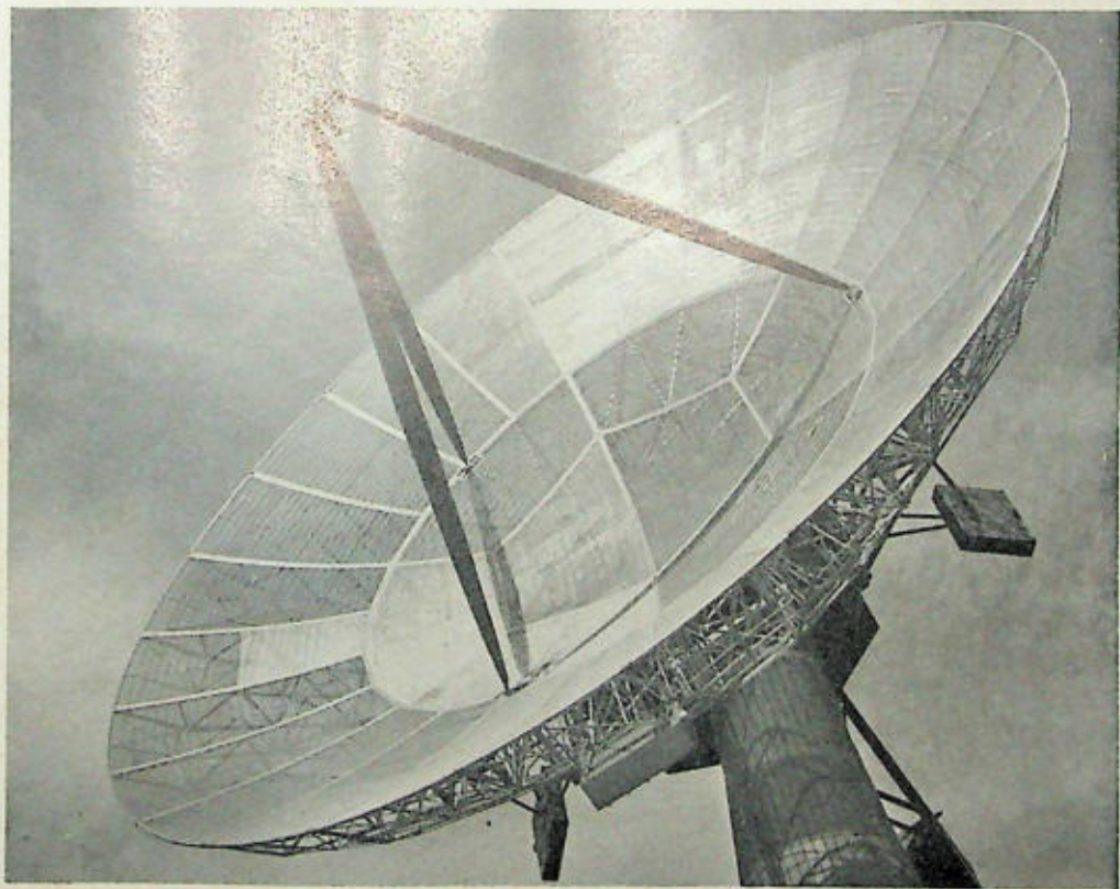
The 60-foot George R. Agassiz radio telescope. (Photograph by Robert E. Cox, with permission of Sky and Telescope.)
