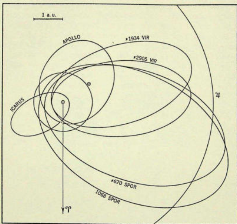
FIGURE 6.—The orbits of two sporadic meteors and two streams of the Virginid shower, with the orbits of the asteroids Icarus and Apollo for comparison.
