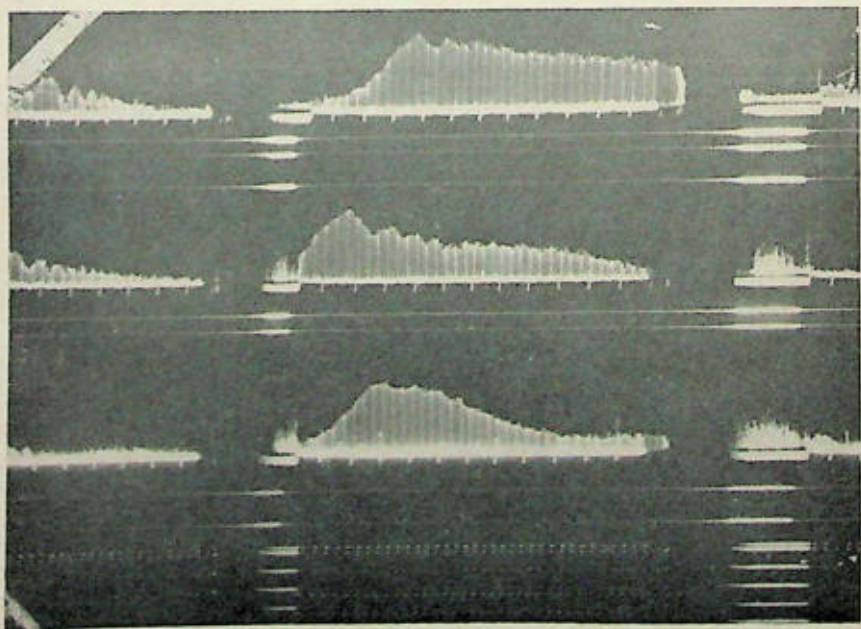
2. Record of radio pulses from a meteor. (J. G. Davies, Jodrell Bank, England.)
