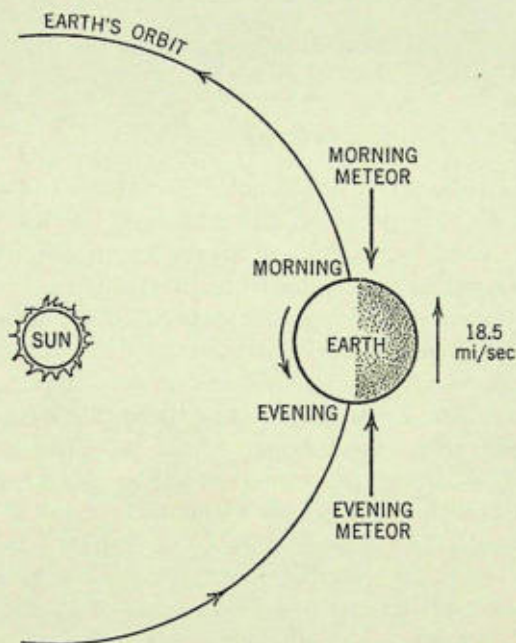
FIGURE 1.—Schematic diagram showing how meteorites collide with the earth.
