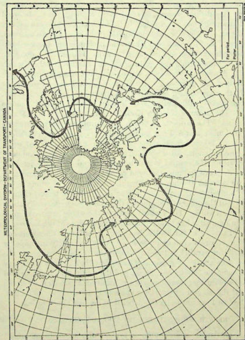
FIGURE 1.—Typical path of the polar jet stream in the Northern Hemisphere.
