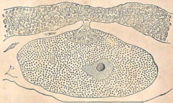
Fig. 872.—Egg-cell of a coral ( Corallimorphus rigidus ), with cells of the nutritive layer (above) projecting into it. Within the egg-cell are seen the large nucleus and numerous yolk-granules. Much enlarged.
