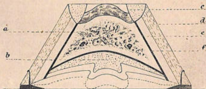
Diagram of vertical cross section of horse's foot to illustrate manner in which seated shoes obtain pressure.
